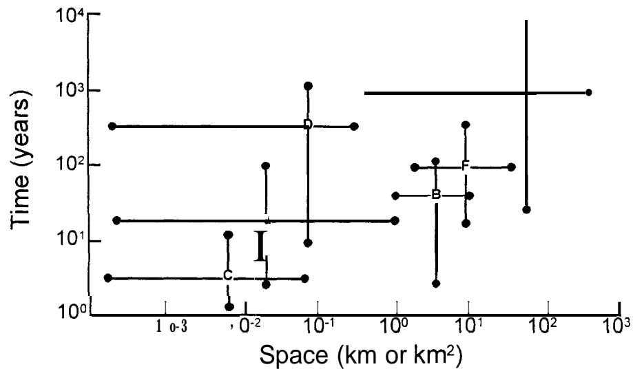
FIGURE 26.1. Illustration of the diversity of spatial and temporal scales influencing the creation and maintenance of riparian forests in the coastal temperate rainforest of North America. Colonization surfaces created by flooding (A), colonization sur-
