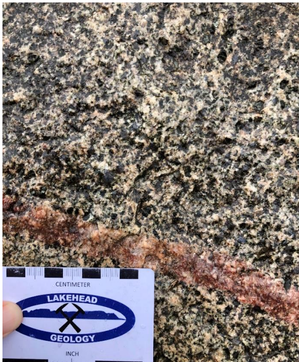
Potassic alteration in the Sabaskong Batholith – Western Wabigoon Subprovince
