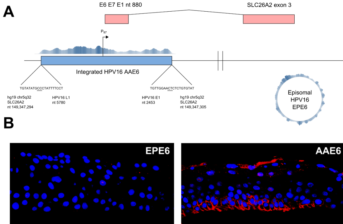
Figure 2.2 – Characterization of viral integration and viral-human fusion transcripts in AAE6 epithelia. [a] Integration site schematic showing viral and human junctions, including nucleotide positions, the early promotor, as well as viral-human fusion transcript between HPV16 early region and SLC26A2 exon 3. A coverage plot above the integrated HPV16 genome demonstrates coverage across the junction sites within SLC26A2 (5482 reads across a 4978 nt assembly containing the AAE6 integrated form flanked by 200 nt of SLC26A2), while a circular coverage plot on the right shows the full episomal assembly of the EPE6 episomal form. [b] Immunofluorescence overlays of EPE6 and AAE6 raft cultures (400x magnification). Nuclei are indicated by blue DAPI staining while SLC26A2 is indicated by red fluorescence.
