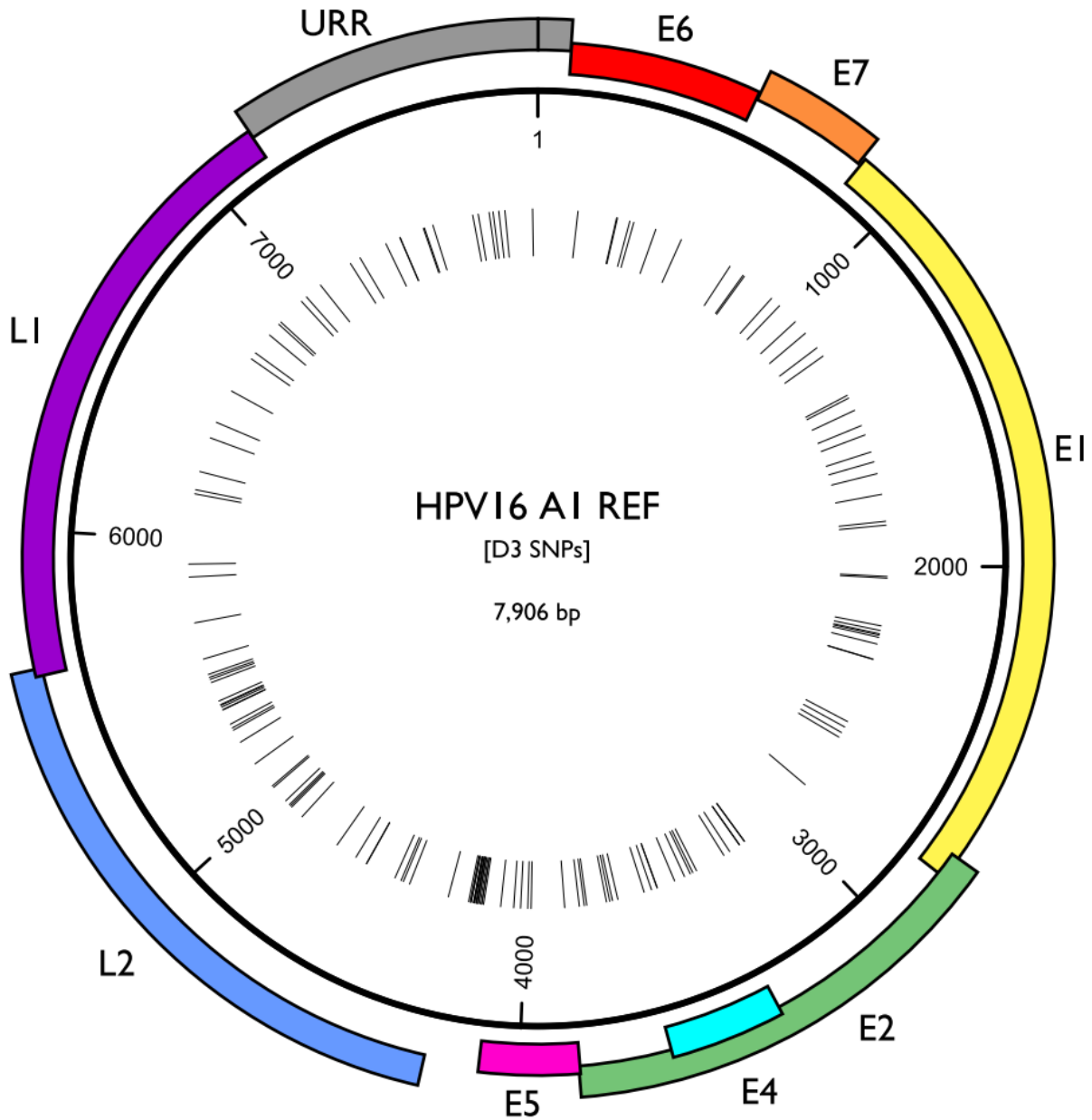
Figure 3C.1 – HPV16 A1 vs D3 single-nucleotide polymorphisms (SNPs). The circular genome of HPV16 A1 (EP reference sequence, GenBank # K02718) is annotated with genomic features. Black lines in the inner ring represent the 151 SNPs present in the D3 variant sub-lineage (AA, GenBank # AF402678) throughout the entire genome and present in genes (E6 [7 SNPs], E7 [3], E1 [31], E2 and E4 [23], E5 [6], L2 [32], L1 [17]), as well as non-coding regions (short non-coding region [17], URR [15]). Circular visualization was created using Circos [Krzywinski et al. , 2009].
