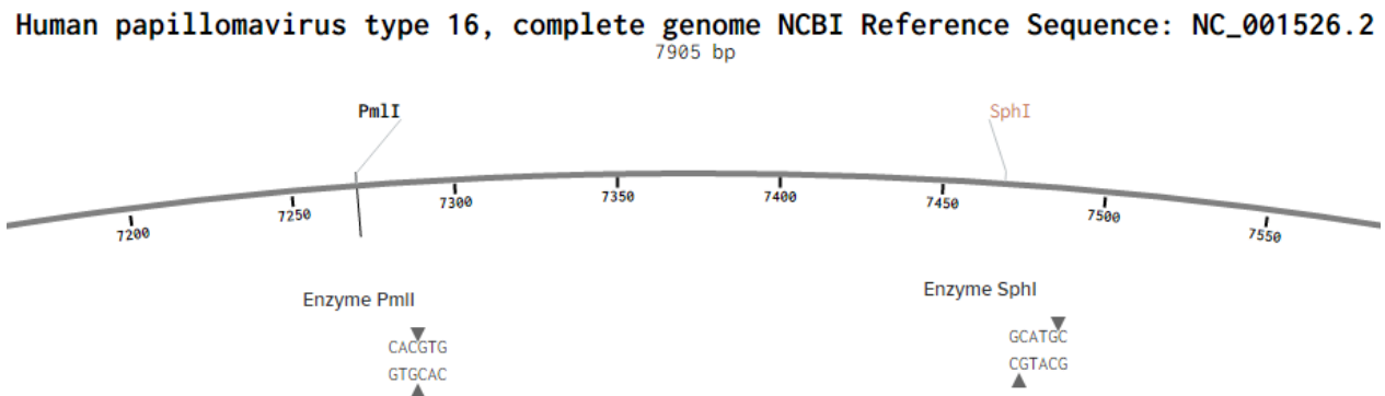
Figure 3C.3 – Location of preferred LoxP sites in HPV16’s URR. PmlI and SphI restriction sites are shown in the non-coding URR of HPV16’s genomes. Image was constructed using Benchling Biology Software.
