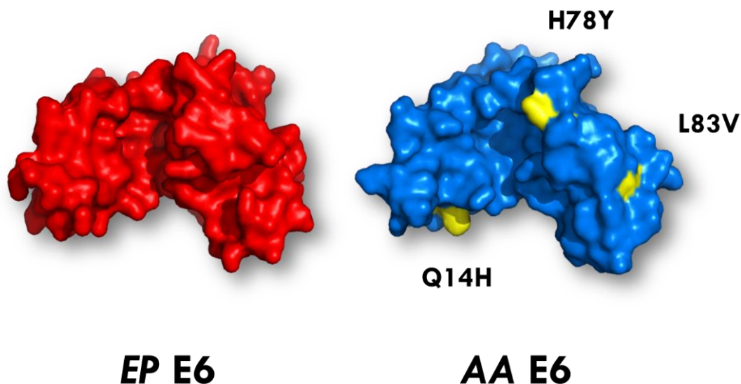
Figure 3C.2 – Predicted 3D protein structures for EP (A1, red) and AA (D2/D3, blue). Pyre2 (intensive mode) [Kelley and Sternberg, 2009; Kelley et al. , 2015] was used for in silico prediction of the 3D protein structures for EP E6 (GenBank #AAA46939.1) and AA E6 (GenBank #AAV91644.1). The sequences were used to generate a 3D model file (.pdb) based on the 151-residue version of E6, starting at the 2 nd Met residue. The 3D models were visualized using PyMOL [The PyMOL Molecular Graphics System, Version 2.0 Schrödinger, LLC]. Amino acid residue differences numbered based on the 151-residue version of E6 are highlighted in yellow (Q14H/H78Y/L83V), causing subtle changes to the protein structure and potential functions.
